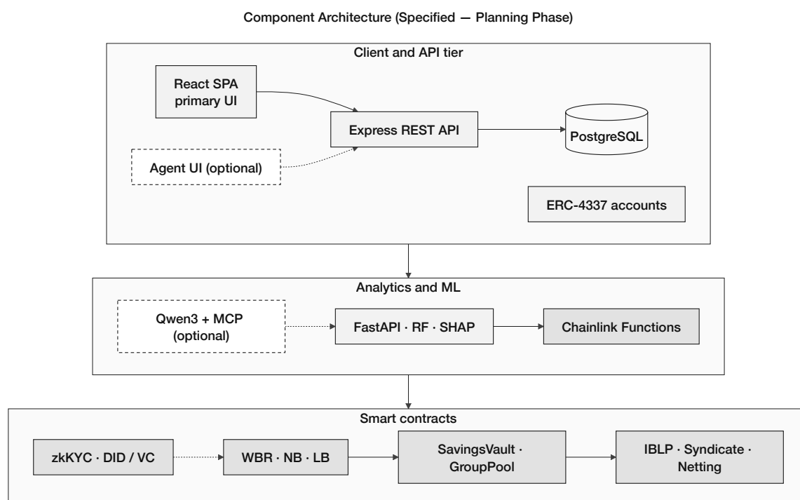
Figure 3.2: Component diagram (planning phase): React UI is the primary path; optional MCP agent (dashed) shares the Express.js API; smart contracts and Chainlink integrations are specified for Phase I–IV deployment.
