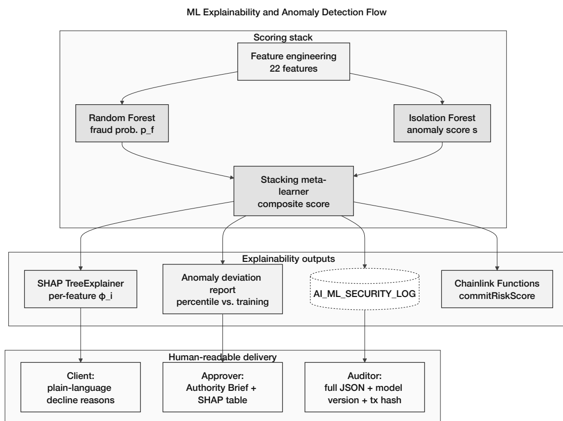
Figure 4.4: Explainability and anomaly-detection flow: feature engineering → Random Forest ( p_f ) + Isolation Forest (anomaly s ) → stacking meta-learner → SHAP + deviation report → three audiences (client, approver, auditor) → oracle commit; human approver retains final disbursement authority.
