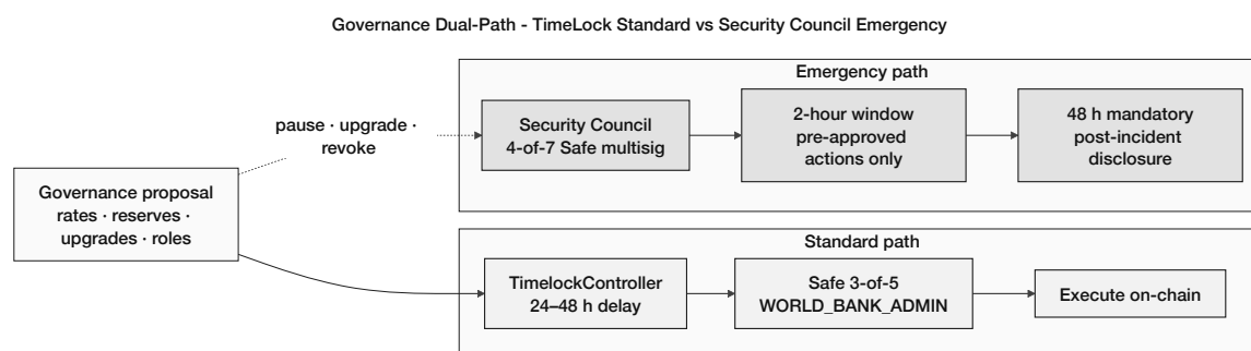
Figure 3.28: Governance dual-path: (a) standard TimeLock-gated parameter changes and upgrades via Safe 3-of-5, and (b) Security Council emergency path (4-of-7) for pre-approved pause, upgrade, and role-revocation actions within a 2-hour window with mandatory 48-hour disclosure.
