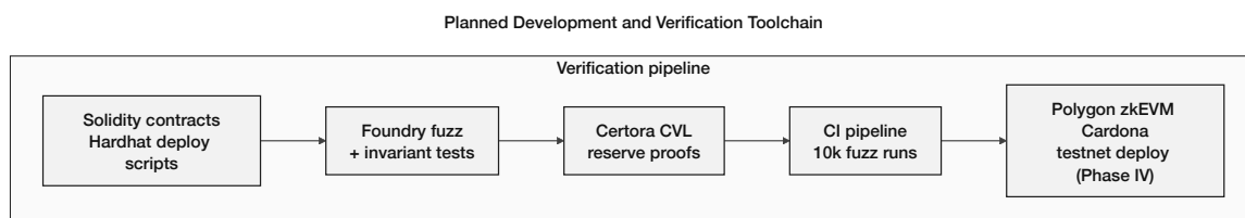
Figure 4.11: Planned development and verification toolchain: Solidity contracts (Hardhat deploy) → Foundry fuzz/invariants → Certora CVL proofs → CI pipeline; testnet deployment to Polygon zkEVM Cardona in Phase IV.
