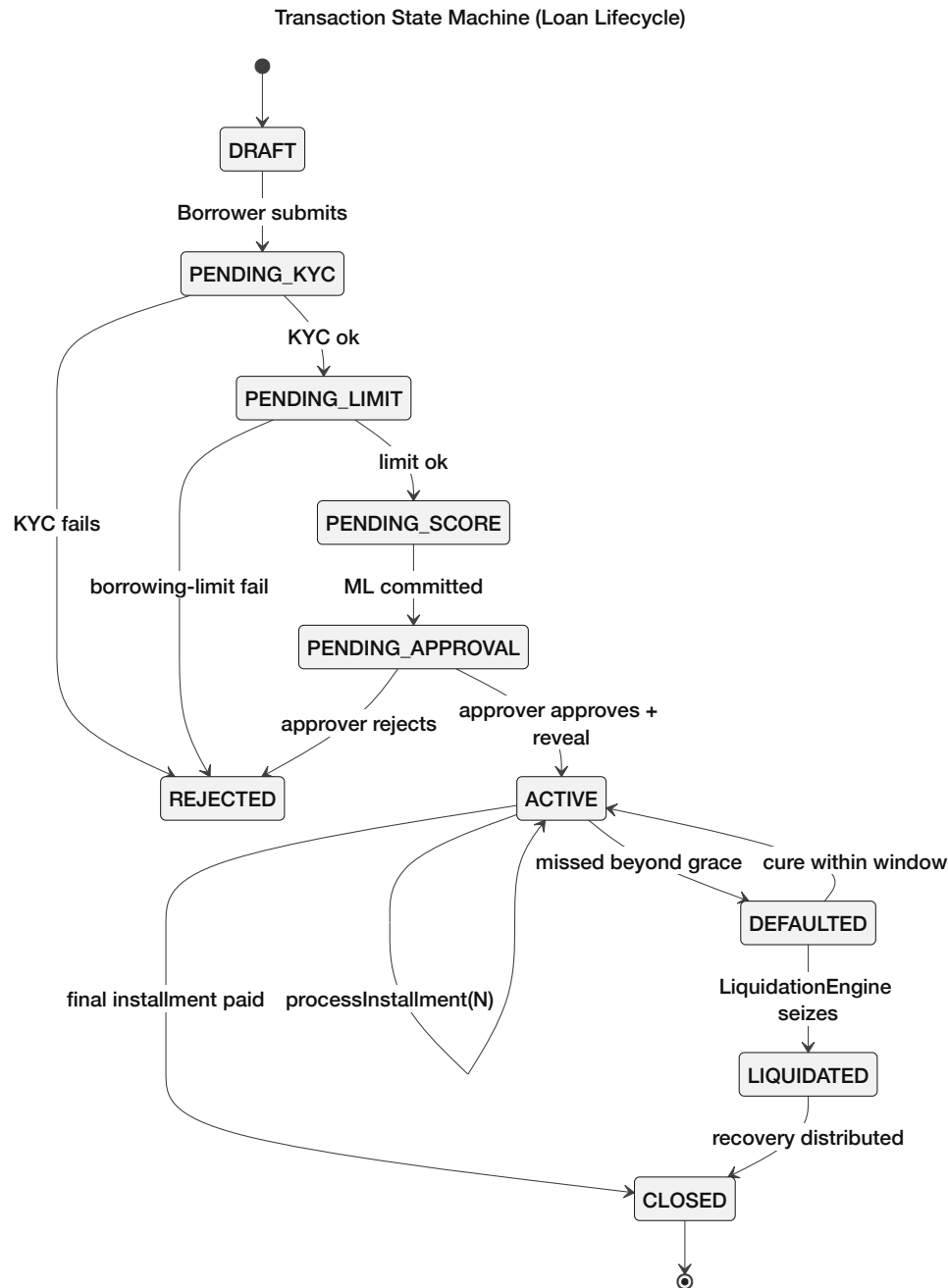
Figure 4.6: Transaction state machine of the loan lifecycle: DRAFT \rightarrow PENDING\_KYC \rightarrow PENDING\_LIMIT \rightarrow PENDING\_SCORE \rightarrow PENDING\_APPROVAL \rightarrow ACTIVE \rightarrow \{CLOSED, DEFAULTED \rightarrow \{LIQUIDATED, \text{cured-back-to-ACTIVE}\}\} , with every transition guarded by a CEI-ordered contract function and every transition emitting an indexed event.
