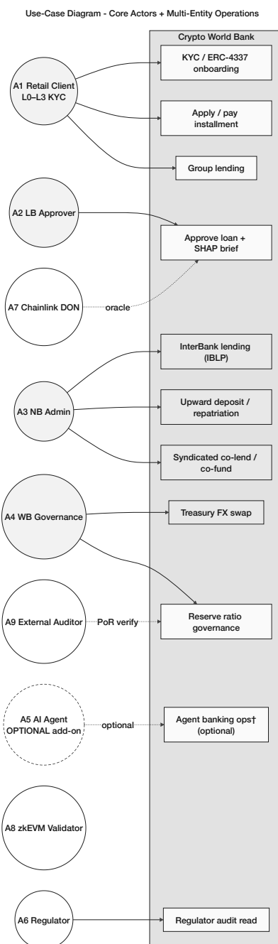
Figure 3.16: Use-case diagram reflecting the nine-actor taxonomy of Table ??: four core primary actors (A1–A4), optional add-on AI Agent (A5, dashed), and four secondary actors (A6–A9). Highlighted use cases cover multi-entity operations (IBLP, upward deposit, syndicated co-lend, treasury FX); optional agent banking ops (UC10) are excluded from MVT.
